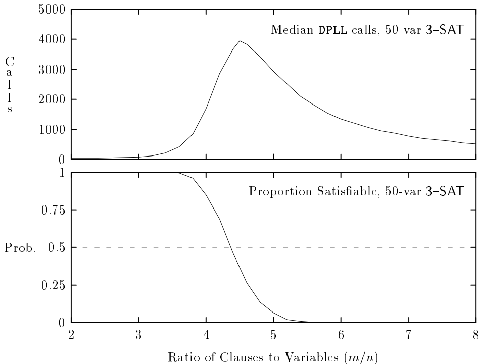
FIGURE 1. Random 3-SAT: DPLL performance and probability of being satisfiable.
